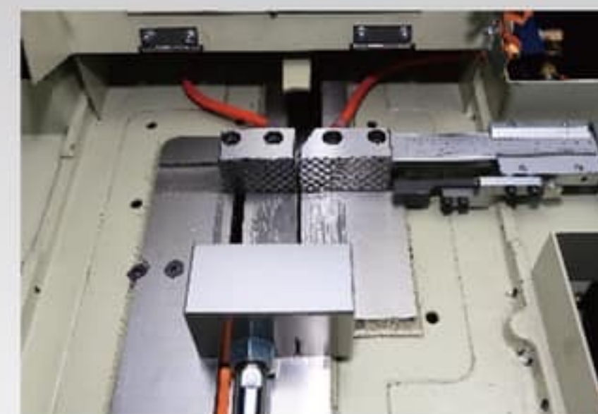
雙邊穩定夾持 Double-side stable clamping
